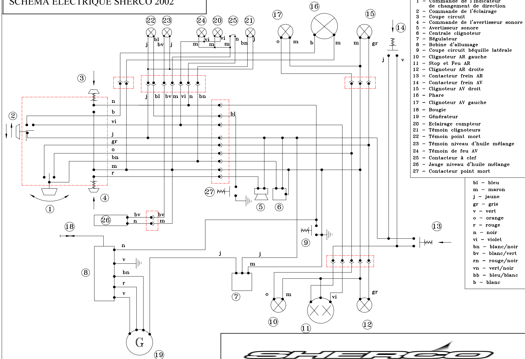
SCHEMA ELECTRIQUE SHERCO 2002
